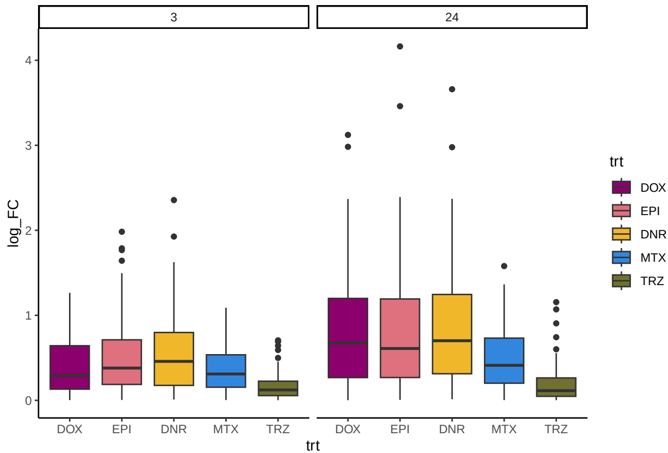
logFC of AF overlapping regions, n = 76
